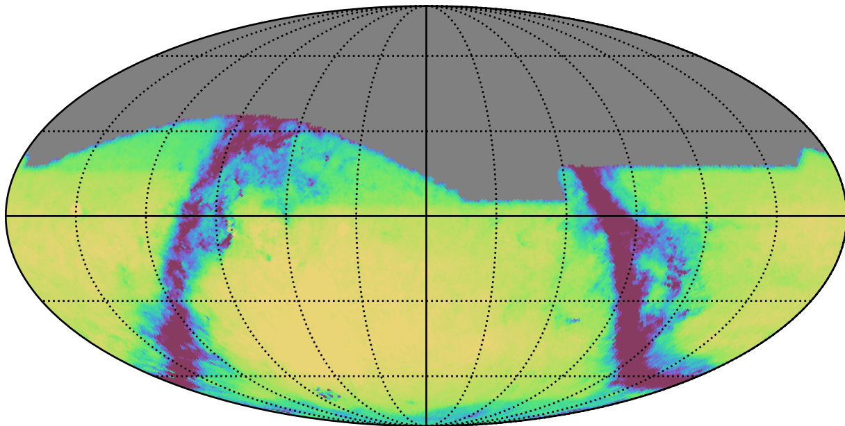
ddf_loaded_fl2_v3.4_10yrs All sky g band: Exgal_CoaddM5
