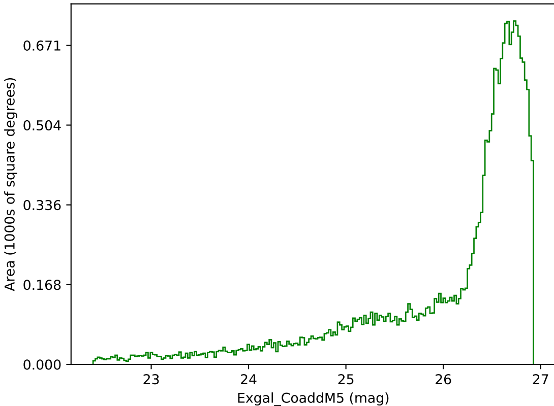
ddf_loaded_fl2_v3.4_10yrs All sky g band: Exgal_CoaddM5
