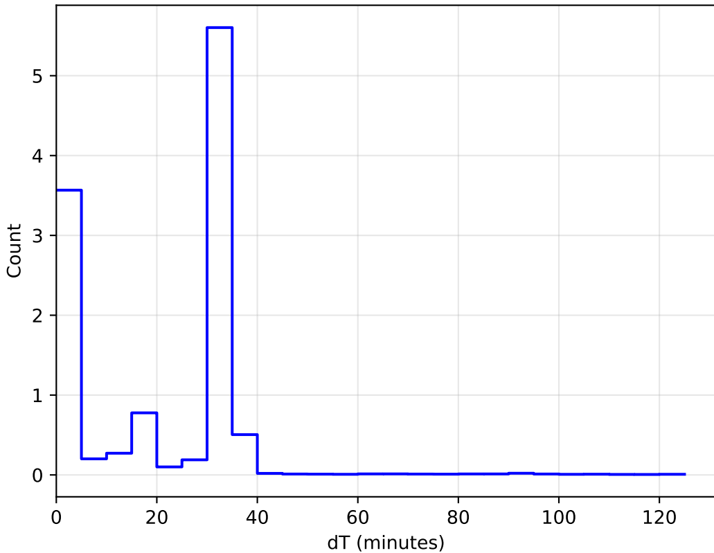
1e6 ddf_loaded_fl2_v3.4_10yrs WFD: DeltaT Histogram
