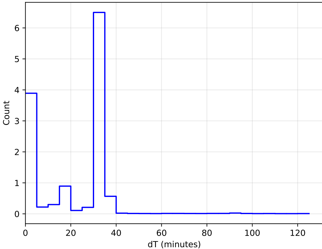
1e6 ddf_loaded_fl2_v3.4_10yrs All sky: DeltaT Histogram
