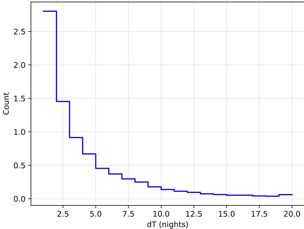
ddf_loaded_fl2_v3.4_10yrs WFD all bands: DeltaNight Histogram 1e6
