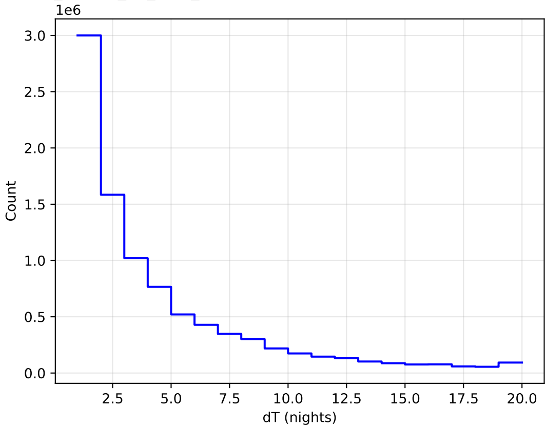
ddf_loaded_fl2_v3.4_10yrs All sky all bands: DeltaNight Histogram
