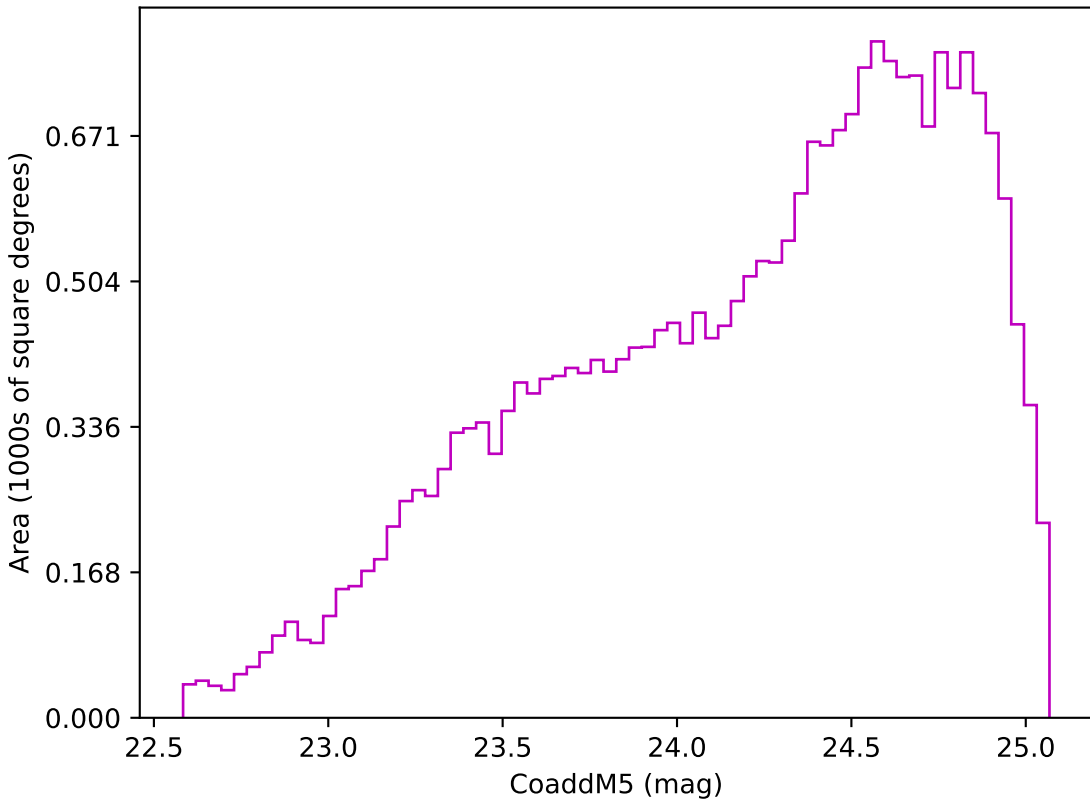
ddf_loaded_fl2_v3.4_10yrs Yr 3-4 z band: CoaddM5
