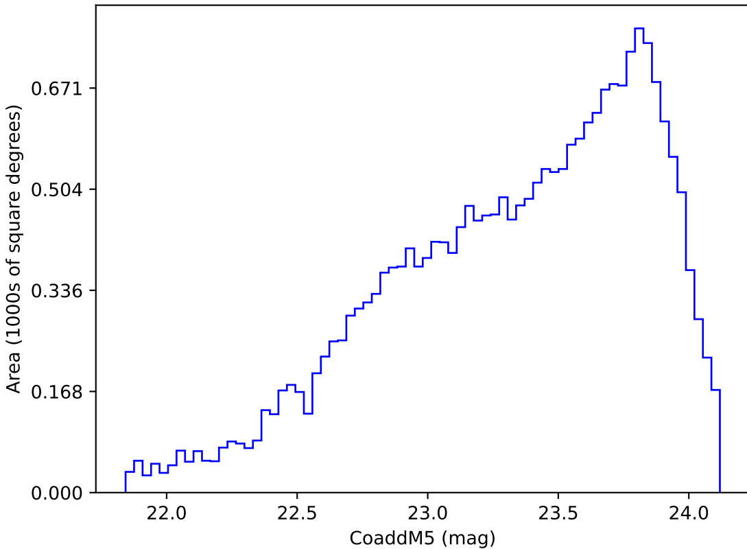
ddf_loaded_fl2_v3.4_10yrs Yr 3-4 y band: CoaddM5
