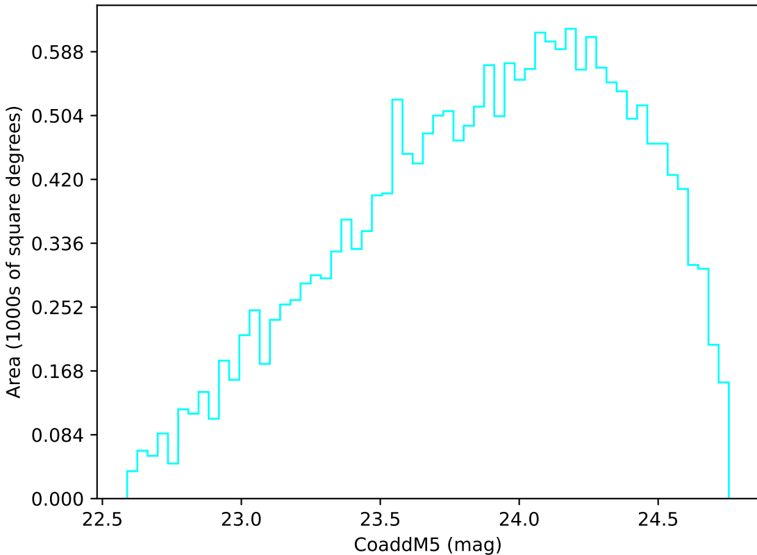
ddf_loaded_fl2_v3.4_10yrs Yr 3-4 u band: CoaddM5
