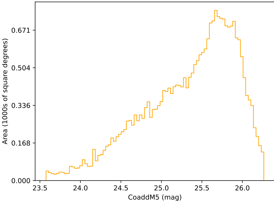
ddf_loaded_fl2_v3.4_10yrs Yr 3-4 r band: CoaddM5
