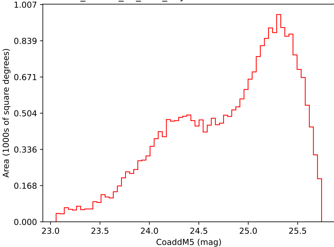
ddf_loaded_fl2_v3.4_10yrs Yr 3-4 i band: CoaddM5
