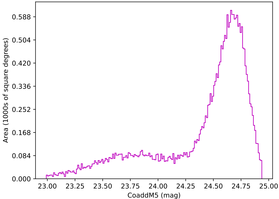
ddf_loaded_fl2_v3.4_10yrs Yr 1 z band: CoaddM5
