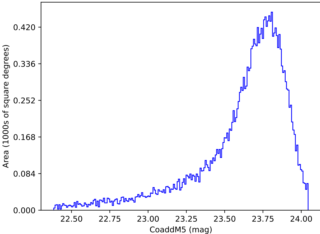
ddf_loaded_fl2_v3.4_10yrs Yr 1 y band: CoaddM5
