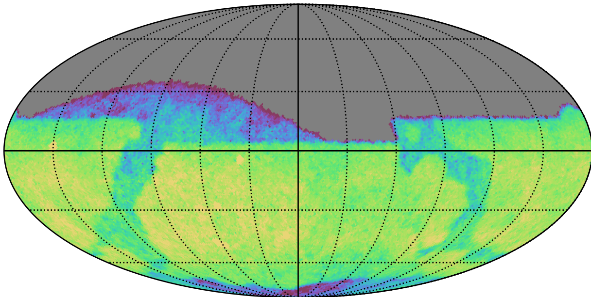
ddf_loaded_fl2_v3.4_10yrs Yr 1 r band: CoaddM5
