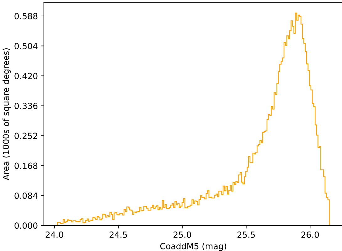
ddf_loaded_fl2_v3.4_10yrs Yr 1 r band: CoaddM5
