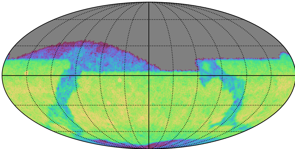
ddf_loaded_fl2_v3.4_10yrs Yr 1 i band: CoaddM5
