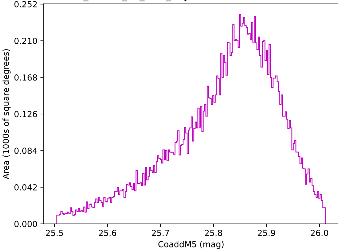
ddf_loaded_fl2_v3.4_10yrs WFD z band: CoaddM5
