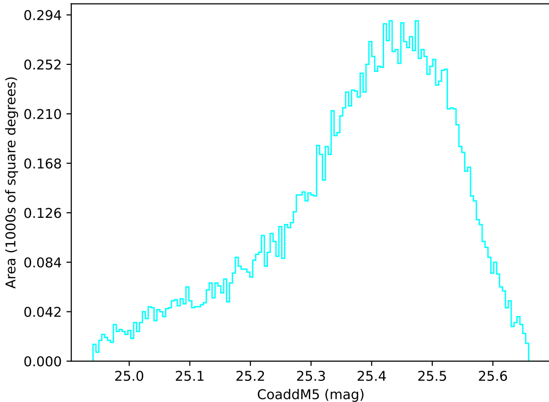
ddf_loaded_fl2_v3.4_10yrs WFD u band: CoaddM5
