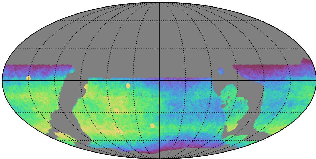
ddf_loaded_fl2_v3.4_10yrs WFD r band: CoaddM5
