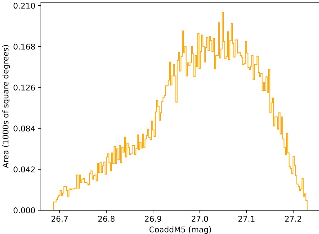
ddf_loaded_fl2_v3.4_10yrs WFD r band: CoaddM5
