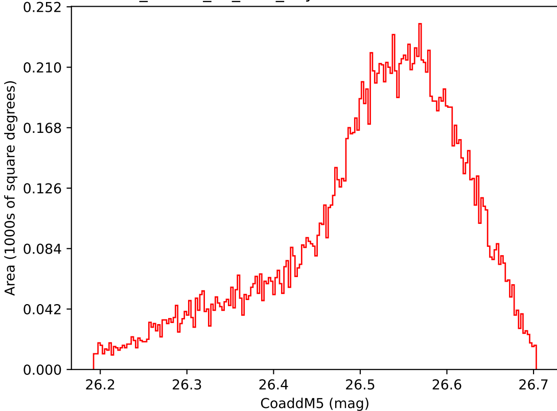
ddf_loaded_fl2_v3.4_10yrs WFD i band: CoaddM5
