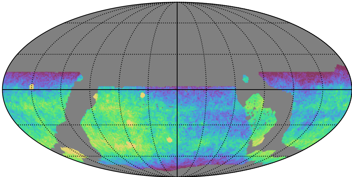
ddf_loaded_fl2_v3.4_10yrs WFD g band: CoaddM5
