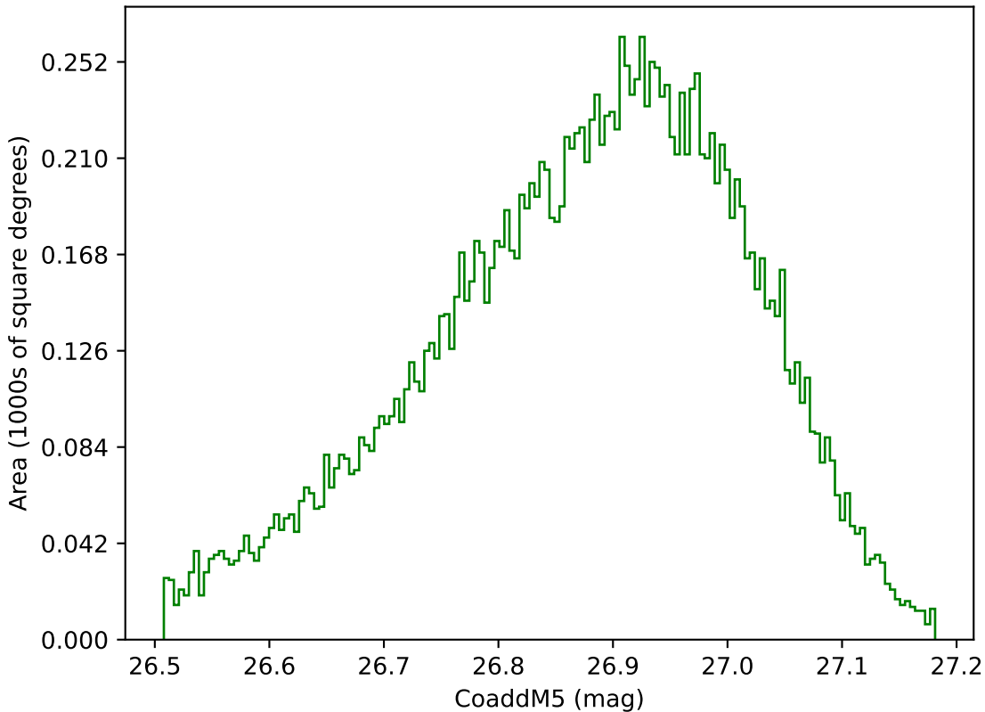
ddf_loaded_fl2_v3.4_10yrs WFD g band: CoaddM5
