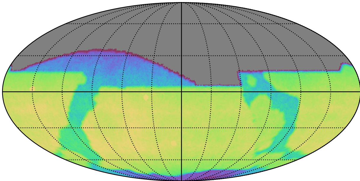
ddf_loaded_fl2_v3.4_10yrs All sky z band: CoaddM5
