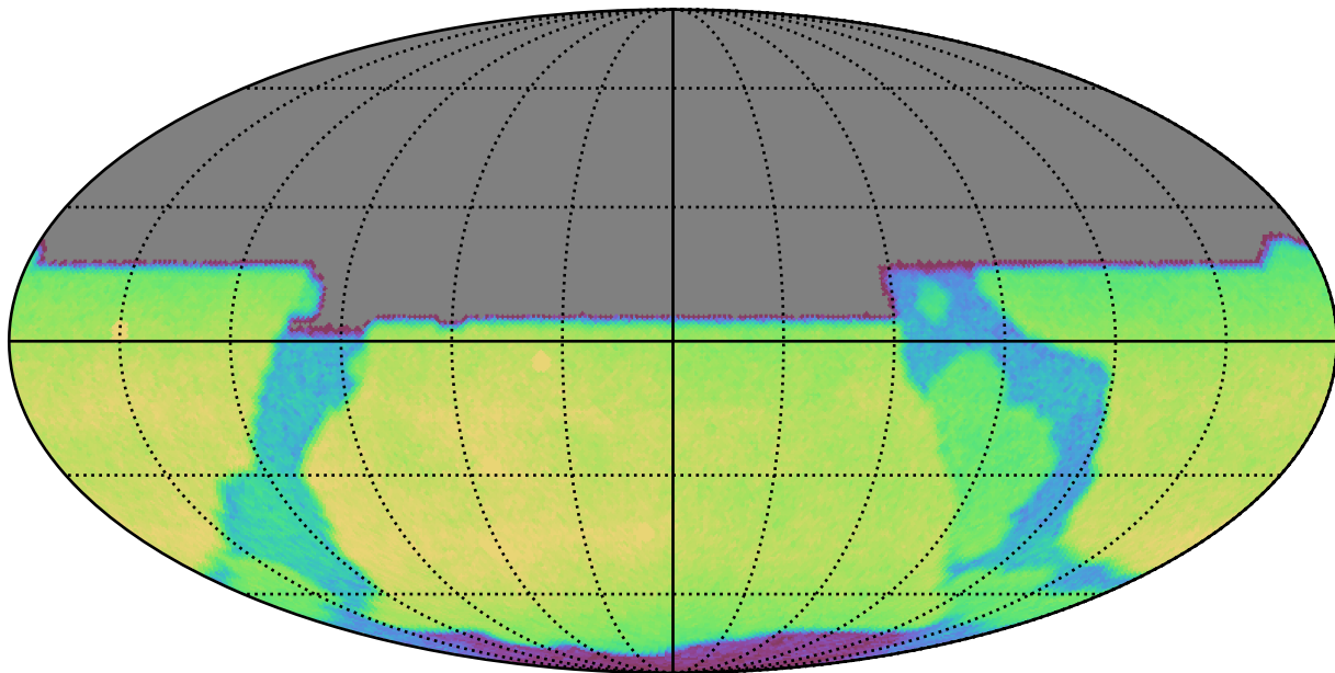
ddf_loaded_fl2_v3.4_10yrs All sky y band: CoaddM5
