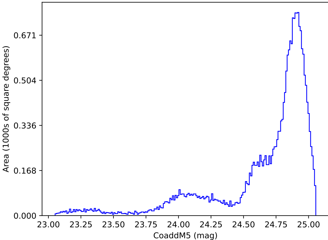
ddf_loaded_fl2_v3.4_10yrs All sky y band: CoaddM5
