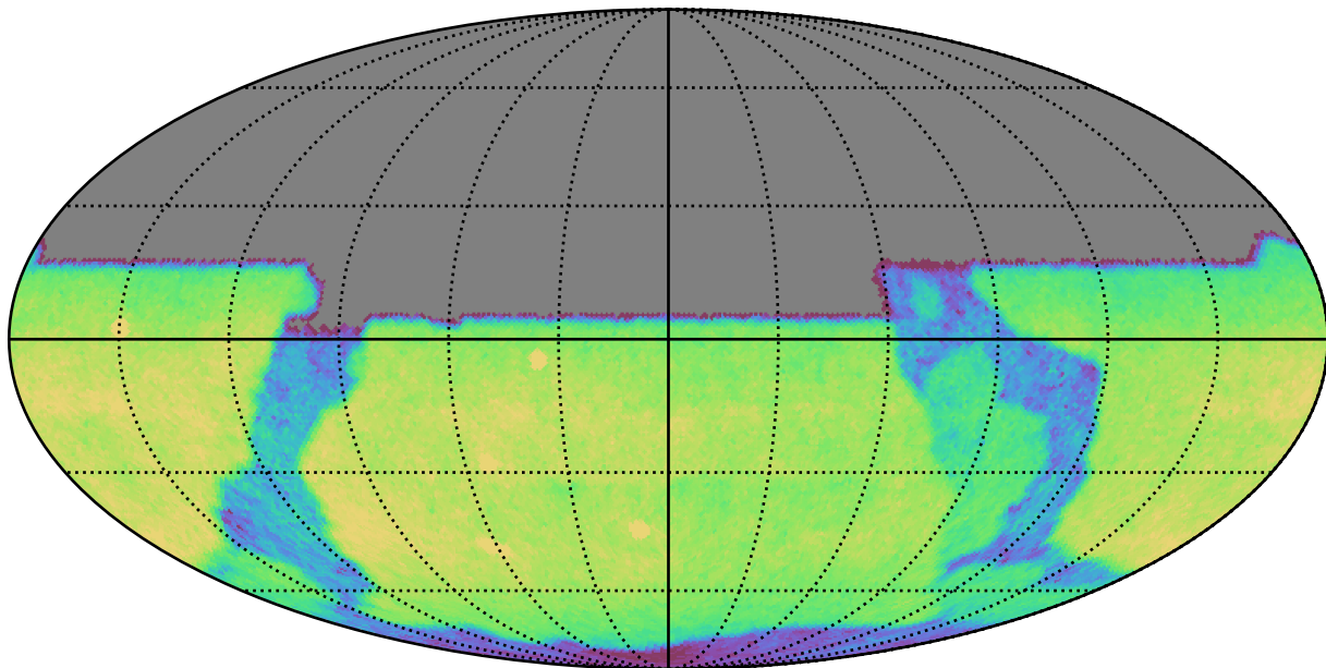
ddf_loaded_fl2_v3.4_10yrs All sky u band: CoaddM5
