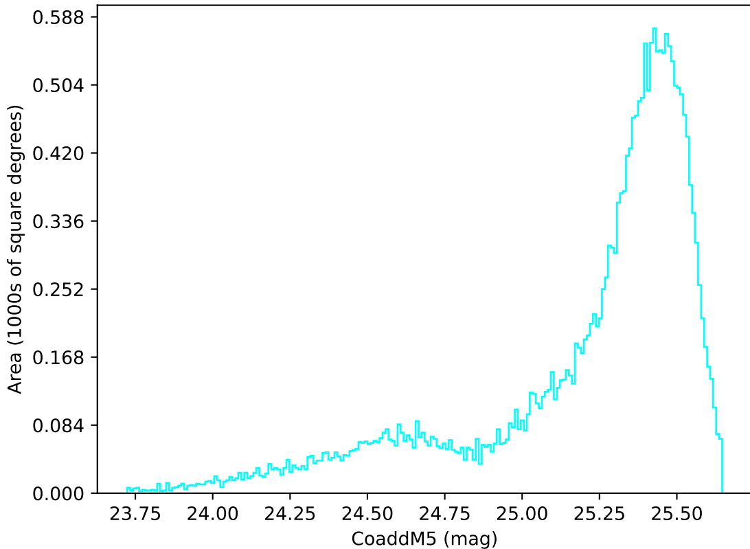
ddf_loaded_fl2_v3.4_10yrs All sky u band: CoaddM5
