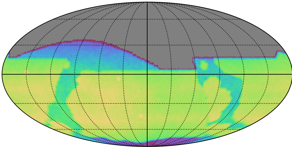
ddf_loaded_fl2_v3.4_10yrs All sky r band: CoaddM5
