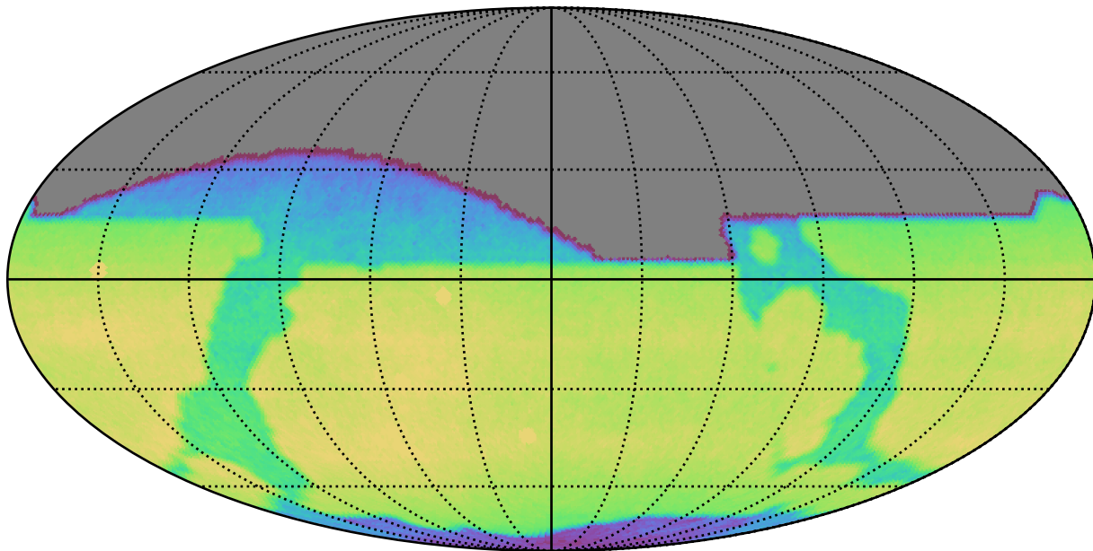
ddf_loaded_fl2_v3.4_10yrs All sky i band: CoaddM5
