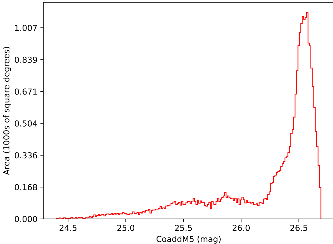
ddf_loaded_fl2_v3.4_10yrs All sky i band: CoaddM5
