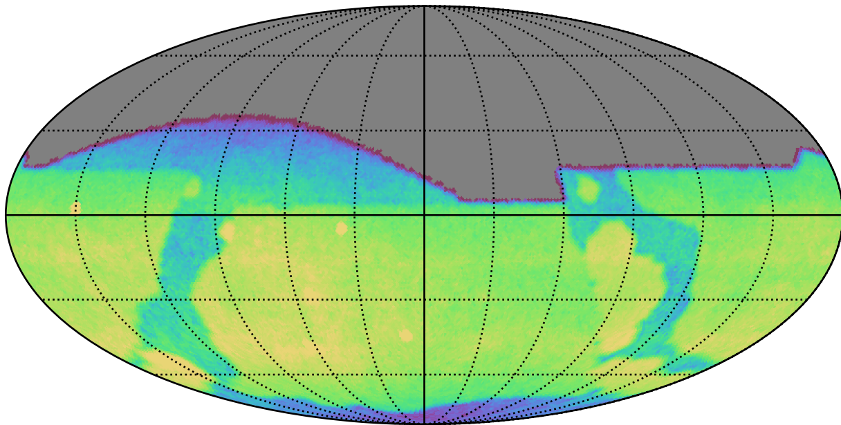
ddf_loaded_fl2_v3.4_10yrs All sky g band: CoaddM5
