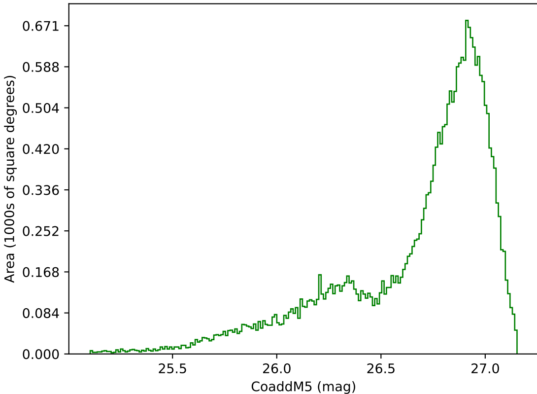
ddf_loaded_fl2_v3.4_10yrs All sky g band: CoaddM5
