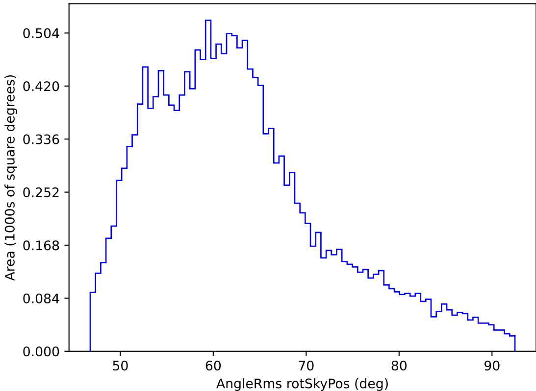
ddf_loaded_fl2_v3.4_10yrs WFD y band: AngleRms rotSkyPos
