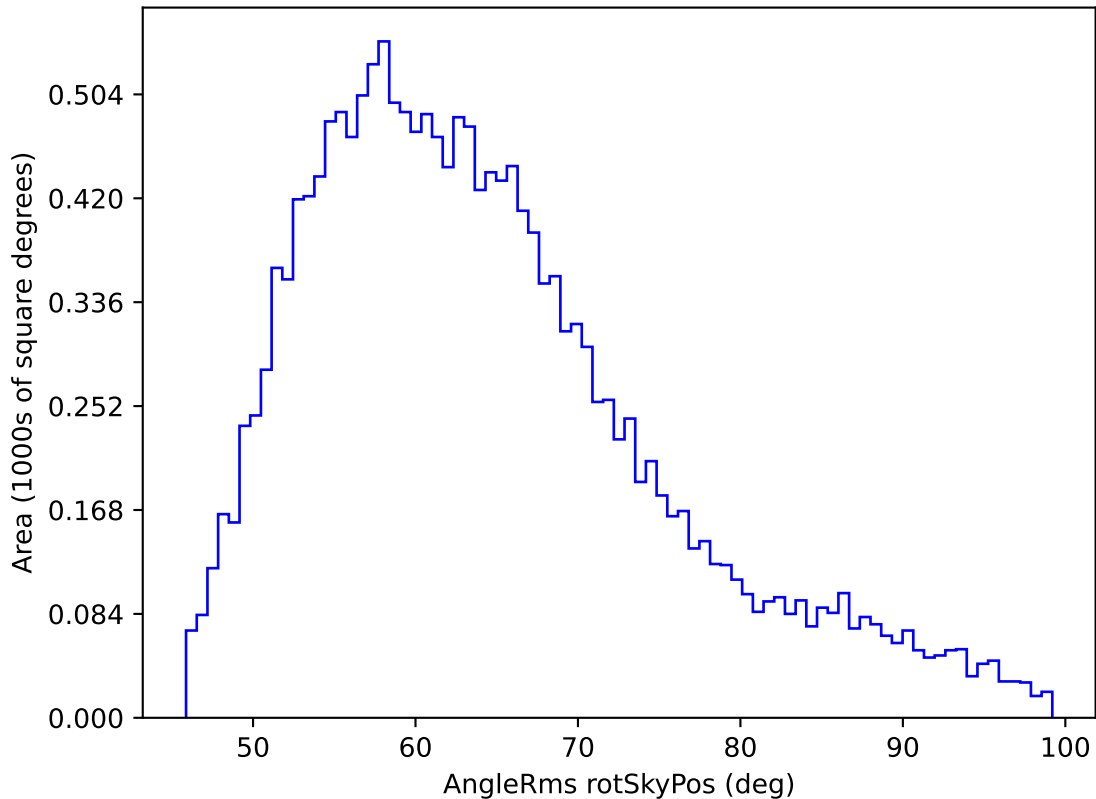
ddf_loaded_fl2_v3.4_10yrs WFD u band: AngleRms rotSkyPos
