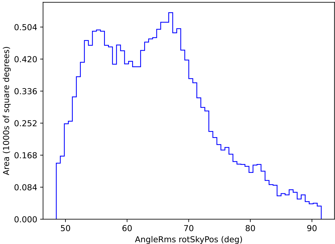
ddf_loaded_fl2_v3.4_10yrs WFD i band: AngleRms rotSkyPos
