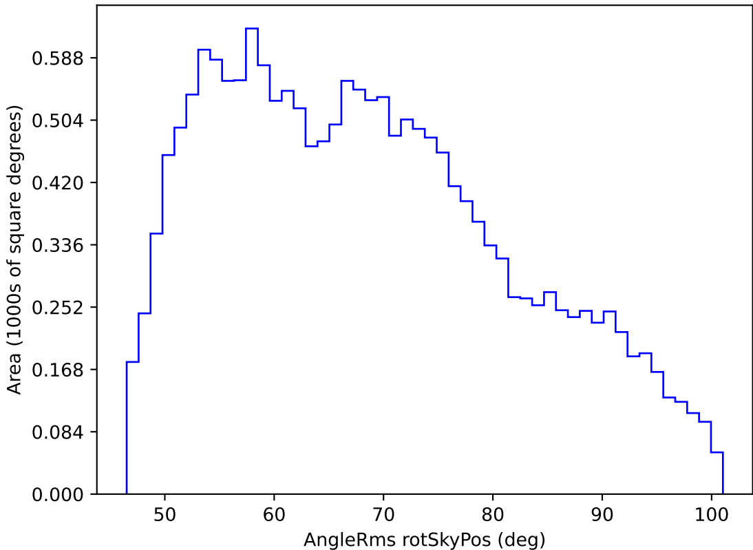
ddf_loaded_fl2_v3.4_10yrs WFD g band: AngleRms rotSkyPos
