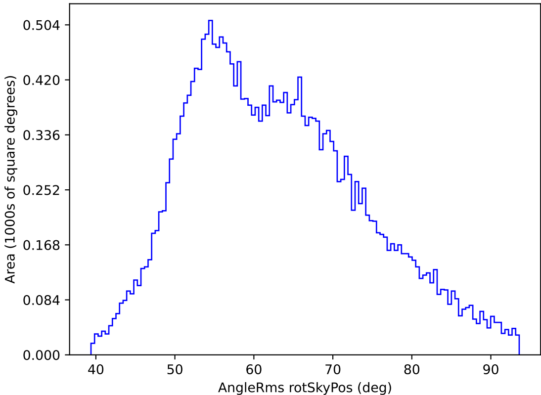
ddf_loaded_fl2_v3.4_10yrs All sky z band: AngleRms rotSkyPos
