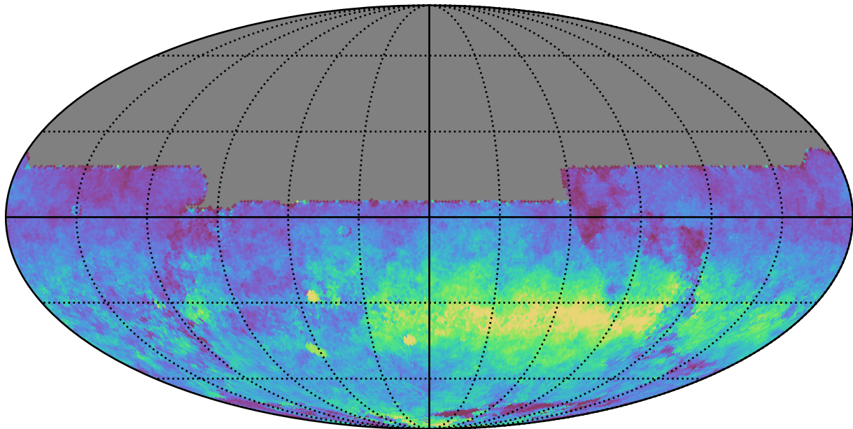
ddf_loaded_fl2_v3.4_10yrs All sky y band: AngleRms rotSkyPos
