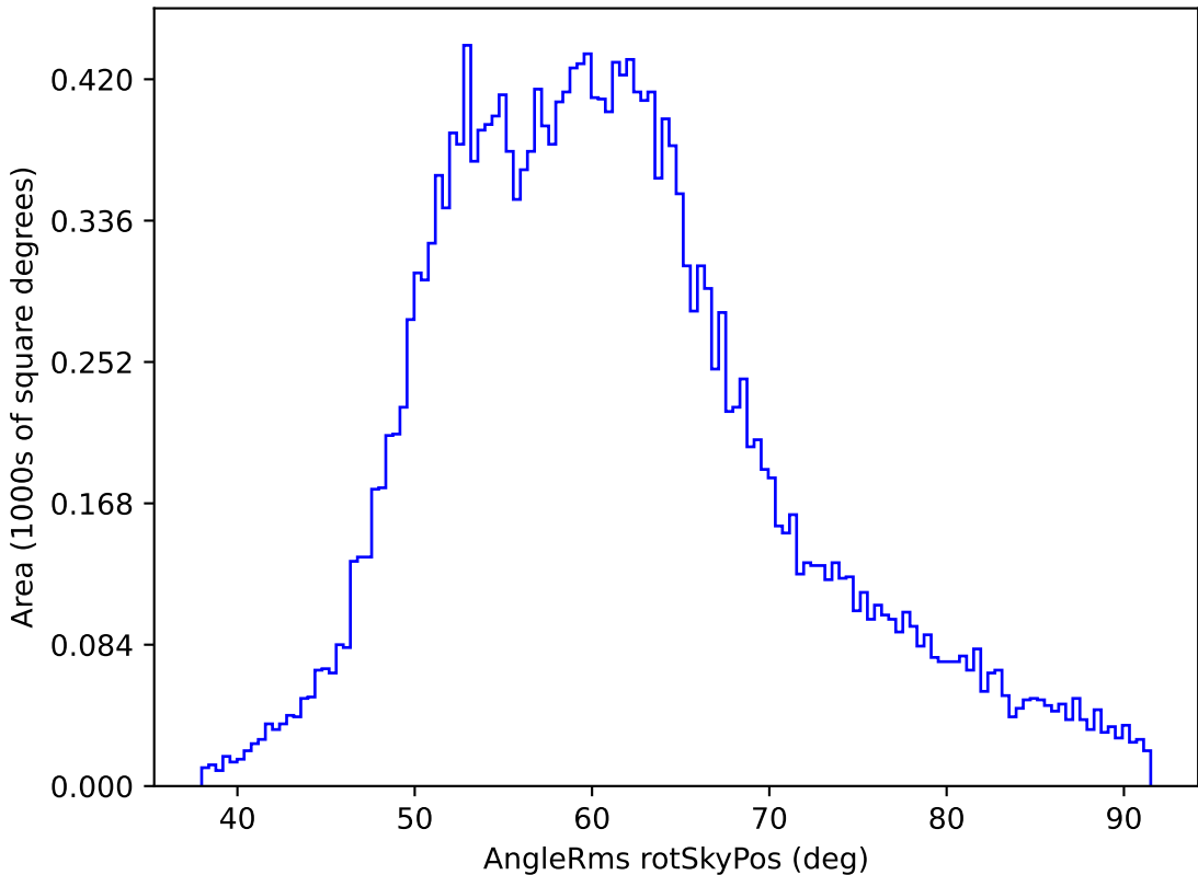
ddf_loaded_fl2_v3.4_10yrs All sky y band: AngleRms rotSkyPos
