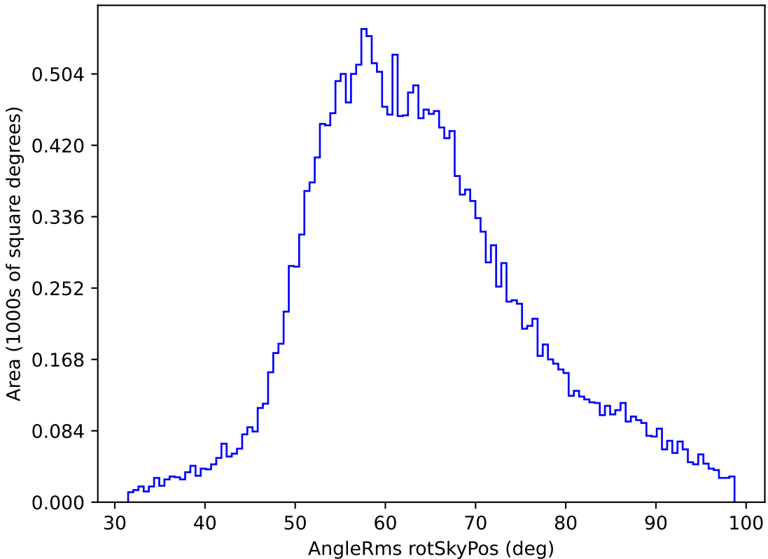
ddf_loaded_fl2_v3.4_10yrs All sky u band: AngleRms rotSkyPos
