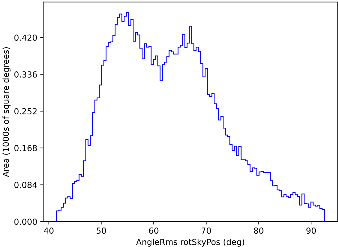
ddf_loaded_fl2_v3.4_10yrs All sky i band: AngleRms rotSkyPos
