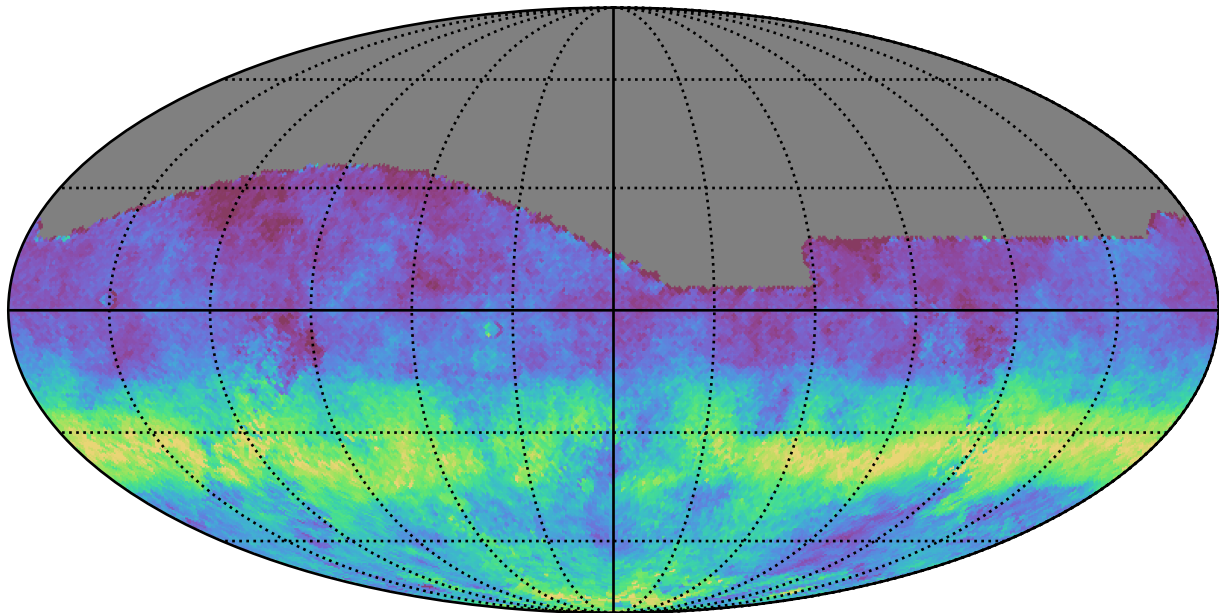
ddf_loaded_fl2_v3.4_10yrs All sky g band: AngleRms rotSkyPos
