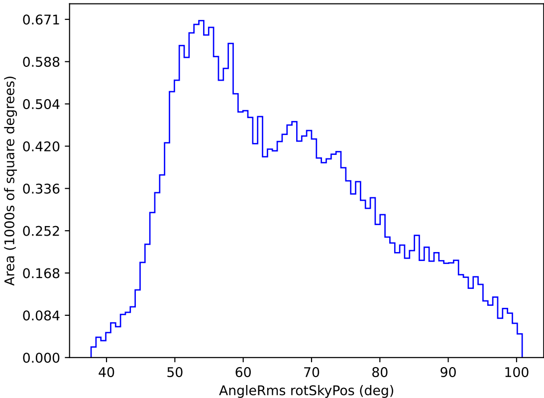
ddf_loaded_fl2_v3.4_10yrs All sky g band: AngleRms rotSkyPos
