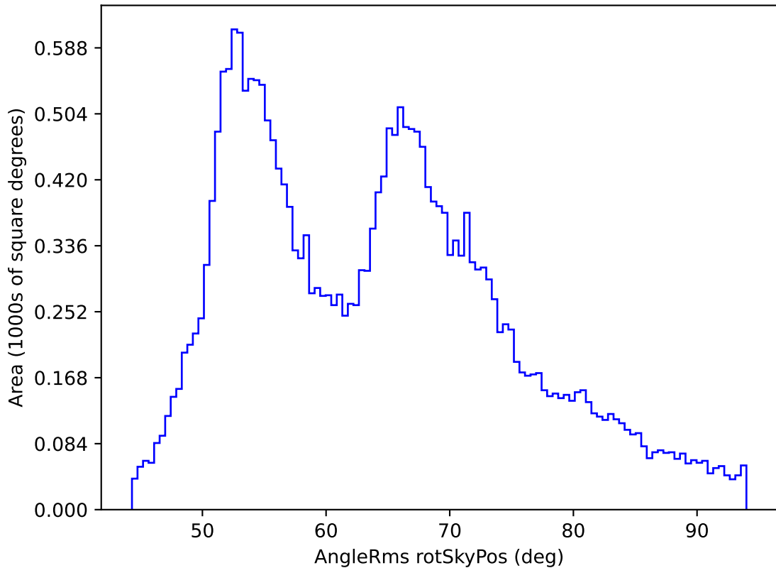
ddf_loaded_fl2_v3.4_10yrs All sky all bands: AngleRms rotSkyPos
