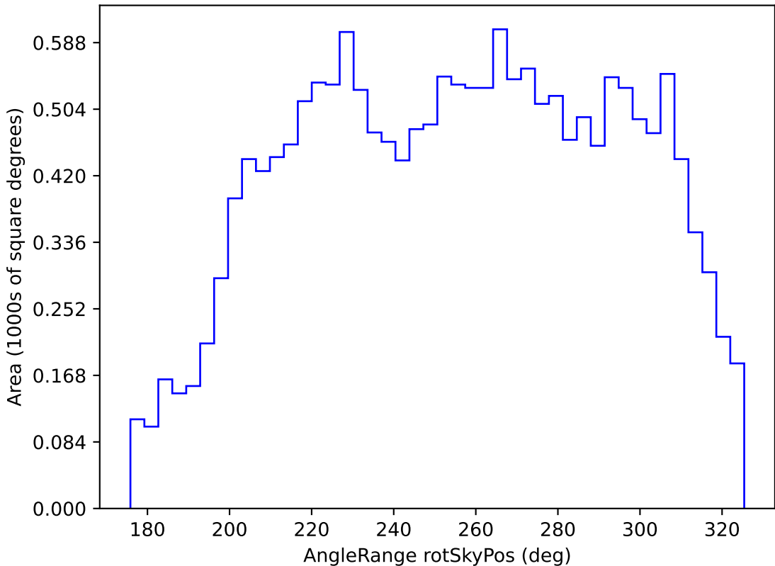
ddf_loaded_fl2_v3.4_10yrs WFD u band: AngleRange rotSkyPos
