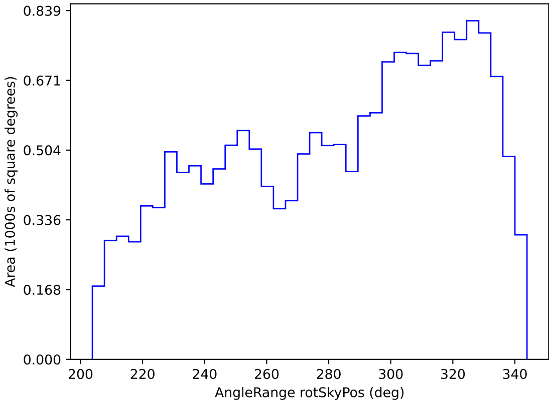
ddf_loaded_fl2_v3.4_10yrs WFD r band: AngleRange rotSkyPos
