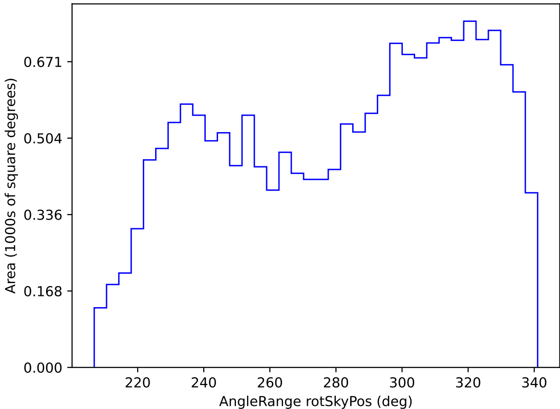
ddf_loaded_fl2_v3.4_10yrs WFD i band: AngleRange rotSkyPos
