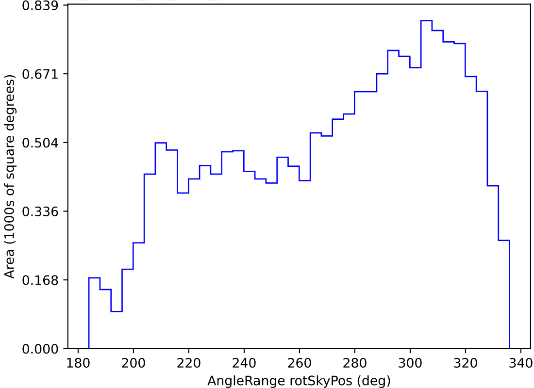
ddf_loaded_fl2_v3.4_10yrs WFD g band: AngleRange rotSkyPos
