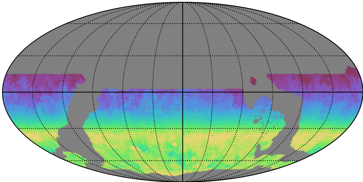
ddf_loaded_fl2_v3.4_10yrs WFD all bands: AngleRange rotSkyPos
